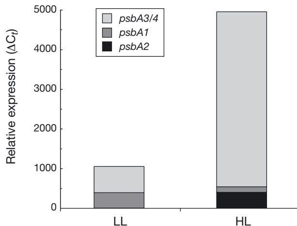
Fig. 6. Absolute changes in the psbA gene pool in Synechococcus WH8102 grown under low-light (LL) and high-light (HL) conditions
