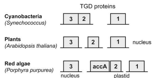
Figure 4. Structural organization of TGD genes in cyanobacteria, plants, and Porphyra . The numbers refer to open reading frames homologous to TGD1, 2, and 3 from Arabidopsis . In Arabidopsis all three genes are encoded in the nuclear genome, whereas TGD1 and 2 are encoded in the plastidial genome of Porphyra .
