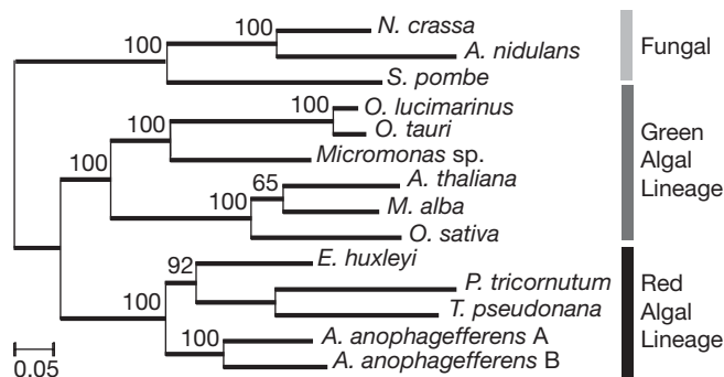
Fig. 4. Unrooted phylogenetic tree of urease protein sequences (approx. 830 amino acids) aligned with the CLUSTAL W multiple sequence alignment algorithm (Thompson et al. 1994) and constructed with MrBayes 3.1 (Ronquist & Huelsenbeck 2003). The scale bar shows number of substitutions per site. Shading as in Fig. 2. Full scientific names are Arabidopsis thaliana , Aspergillus nidulans , Aureococcus anophagefferens , Emiliana huxleyi , Morus alba , Neurospora crassa , Ostreococcus lucimarinus , Oryza sativa , Ostreococcus tauri , Phaeodactylum tricorutum , Schizosaccharomyces pombe and Thalassiosira pseudonana
