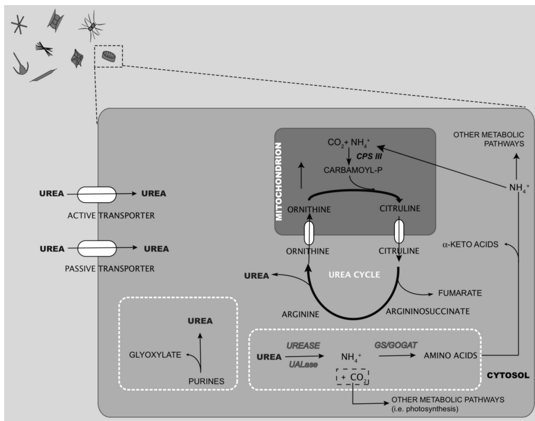
Fig. 1. Urea metabolism pathways. CPS III: carbamoylphosphate synthetase; GS/GOGAT: glutamine synthetase/glutamine: 2-oxoglutarate amidotransferase; UALase: urea amidolyase
