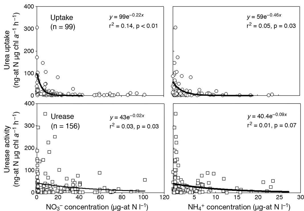
Fig. 3. Urea uptake or urease activity as a function of \text{NO}_3^- concentration and \text{NH}_4^+ concentration in the Chesapeake Bay, USA (from Solomon 2006)
