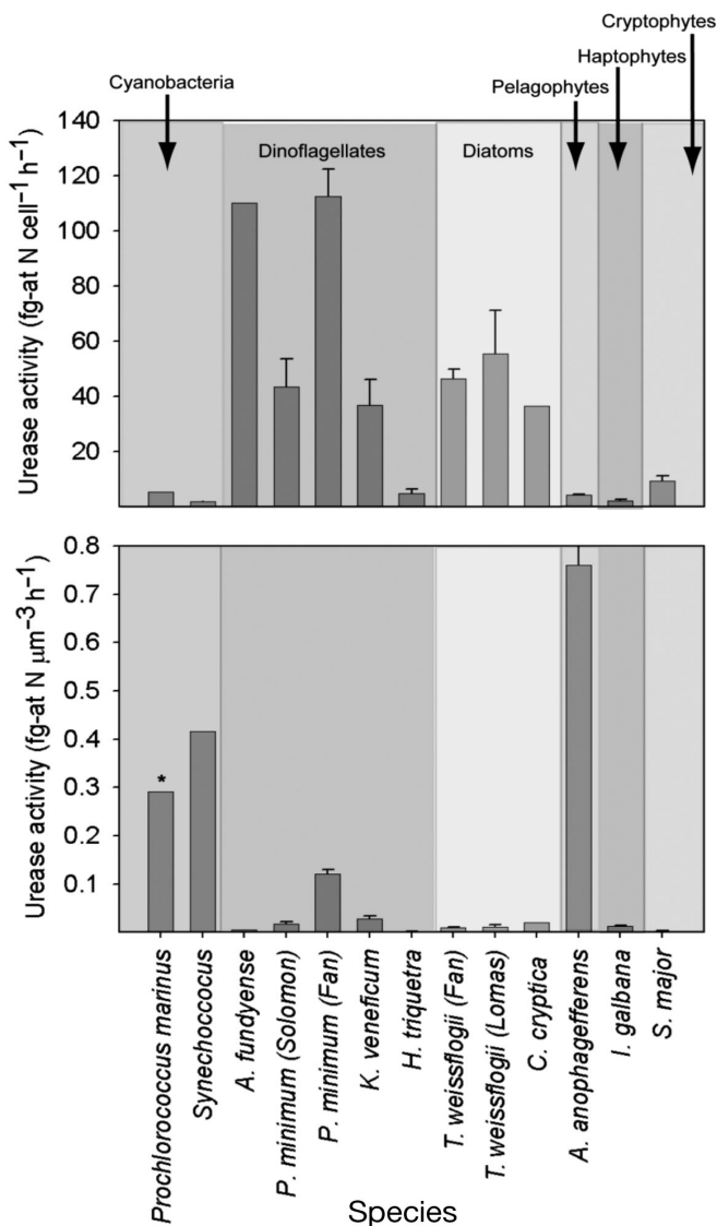
Fig. 6. Comparison of urease activity rates between different phytoplankton species grown on urea on a per cell or per cell volume basis. Data for the Cyanobacteria Prochlorococcus marinus and Synechococcus WH7805 were obtained from Palinska et al. (2000) and Collier et al. (1999), respectively. Rates were converted from \mu\text{M} urea hydrolyzed \text{min}^{-1} protein -1 to \text{fg-at N cell}^{-1} \text{h}^{-1} using 21.5 \text{ fg protein cell}^{-1} for P. marinus (Zubkov & Tarran 2005) and 500 \text{ fg protein cell}^{-1} for WH7805 (Kramer & Morris 1990). P. marinus on a per cell volume basis (*) was divided by 10 to allow for visualization of other species. Data sources of other species are described in Fig. 5. Cell volumes were calculated assuming a sphere or cylinder and diameters obtained from readings on the Coulter Counter or from CCMP. Full scientific names are Alexandrium fundyense , Aureococcus anophagefferens , Cyclotella cryptica , Heterocapsa triquetra , Isochrysis galbana , Karlodinium veneficum , Prorocentrum minimum , Storeatula major and Thalassiosira weissflogii
