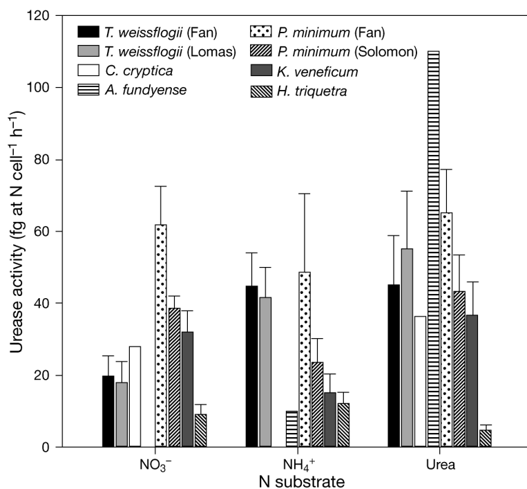
Fig. 5. Comparison of rates of urease activity in diatoms and dinoflagellates grown on different N substrates. Data for the diatoms Thalassiosira weissflogii were obtained from Fan et al. (2003a) and Lomas (2004), and Cyclotella cryptica from Oliveira & Antia (1986). Data for the dinoflagellates Alexandrium fundyense were obtained from Dyhrman & Anderson (2003), Prorocentrum minimum from Fan et al. (2003a), and P. minimum , Karlodinium veneficum , and Heterocapsa triquetra from Solomon & Glibert (2008). Some rates were converted from \mu\text{M} urea hydrolyzed \text{min}^{-1} protein ^{-1} to \text{fg-at N cell}^{-1} \text{h}^{-1} using the regression from Menden-Duer & Lessard (2000) to obtain \text{N cell}^{-1} and due to the fact that from 70 to 90% of cellular N is protein (Wheeler 1983).
