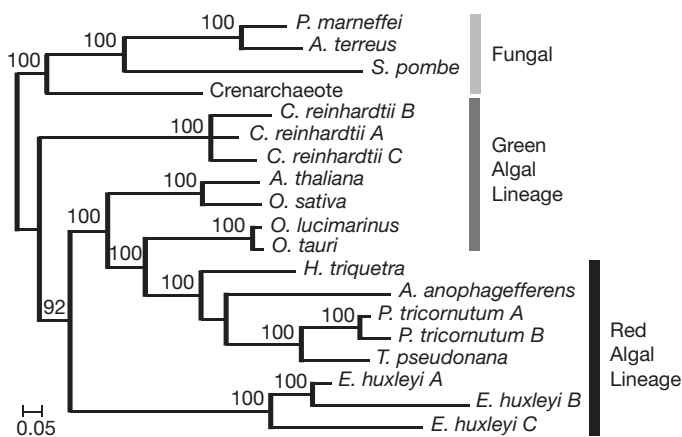
Fig. 2. Unrooted phylogenetic tree of DUR3 protein sequences (approx. 700 amino acids) aligned with the CLUSTAL W multiple sequence alignment algorithm (Thompson et al. 1994) and constructed with MrBayes 3.1 (Ronquist & Huelsenbeck 2003). The scale bar shows number of substitutions per site. The protein sequence of Heterocapsa triquetra was created from 4 separate expressed sequence tag (EST) sequences deposited in GenBank. Dark shading indicates red algal lineages, medium gray shading indicates green algal lineages, and light gray shading represents fungal sequences and the Crenarchaeote sequence. Full scientific names are Arabidopsis thaliana , Aspergillus terreus , Aureococcus anophagefferens , Chlamydomonas reinhardtii , Emiliana huxleyi , Heterocapsa triquetra , Ostreococcus lucimarinus , Oryza sativa , Ostreococcus tauri , Penicillium marneffeii , Phaeodactylum tricornutum , Schizosaccharomyces pombe and Thalassiosira pseudonana
